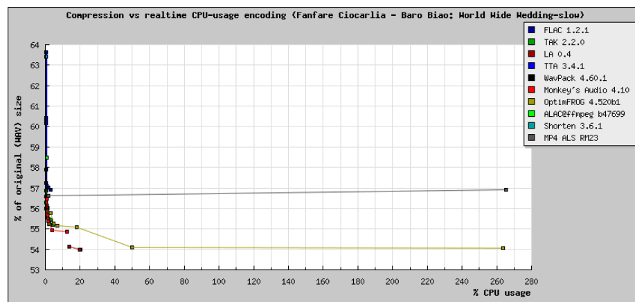
Figure 1.1: Encoding speed as 'calculated CPU-usage' versus compression for 'Fanfare Ciocarlia - Baro Biao: World Wide Wedding'
